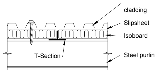
T-Section detail (If purlins exceed recommended spacing for thickness of board)
