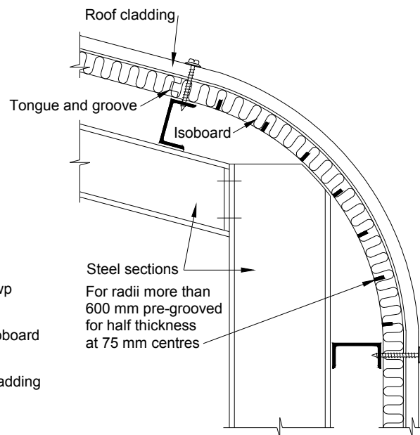
Detail A (Alternative detail)
